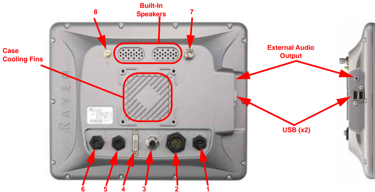
FIGURE 3. Viper 4 Ports and Connectors
